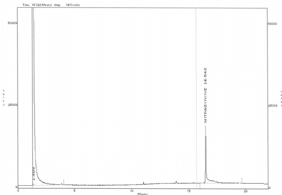
Figure II. Gas chromatogram of mitragynine reference standard
