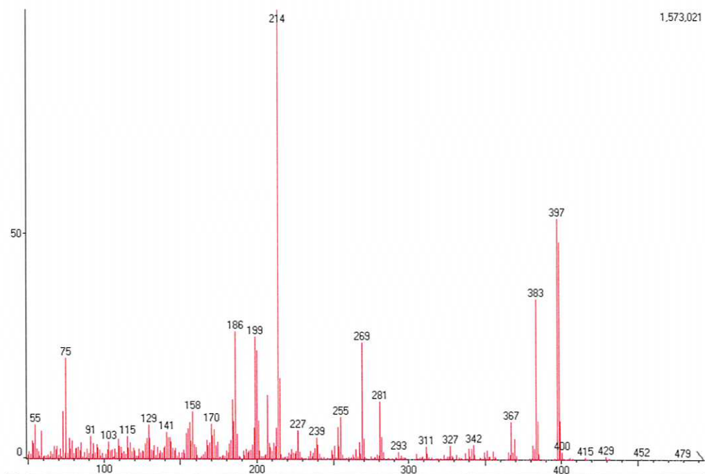
Figure V. Mass spectrum of mitragynine reference standard
