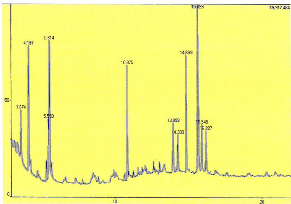
Figure VI. Total ion chromatogram of leaves extract
