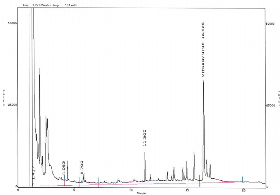
Figure III. Gas chromatogram of leaf extract
